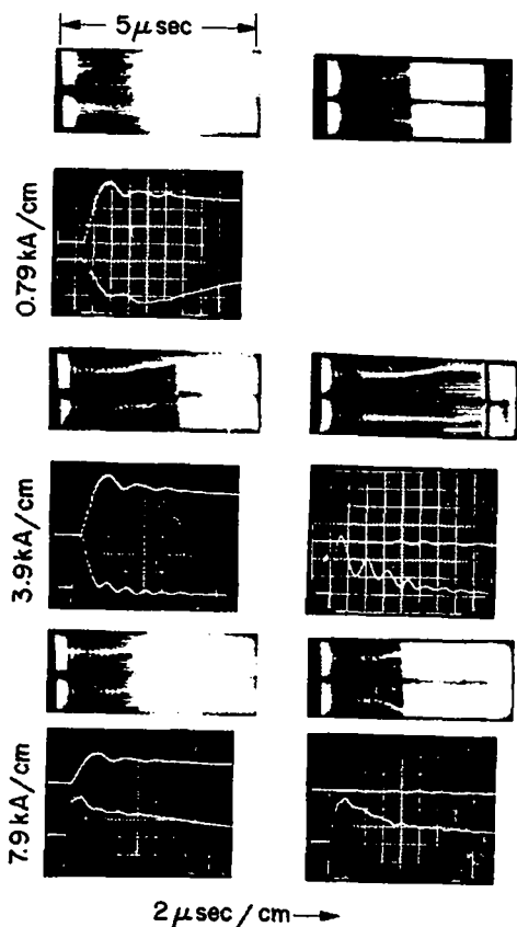
Fig. 4. Streak photographs of m = 1 instability in Scylla IV-3 with 135-cm of \ell = 1 field. The oscillograms show the compression field (top) and the I_z current.
