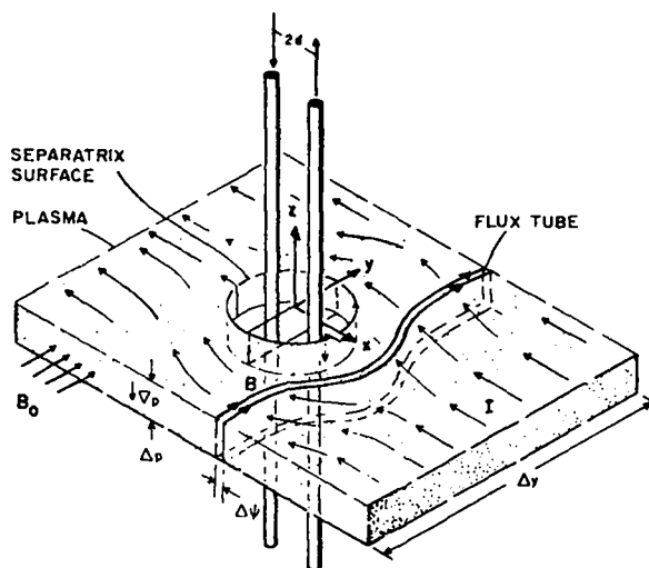
Fig. 51. The geometry of the model.
