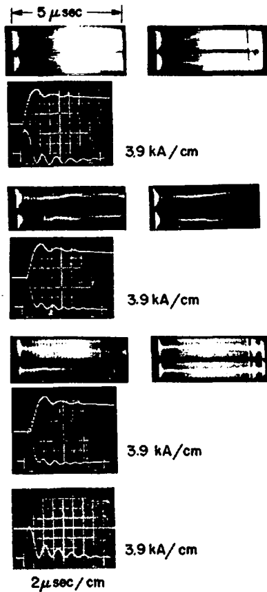
Fig. 5. Streak photographs and oscillograms of Scylla IV-3 as in Fig. 4 with 135-cm of \ell = 1 field.
