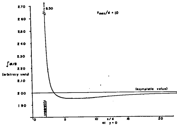
Fig. 52. \int dl/B for a flux line vs the value of x/d at y = 0 for that line.
