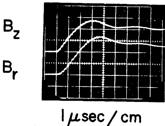
Fig. 2. Oscillograms of Scylla IV-3 compression field (top) and B_r component of \ell = 1 field.
