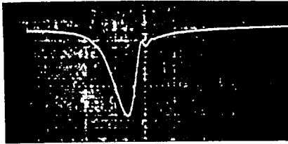
(10 \mu\text{sec} /horizontal division = 0.296 MHz/division) Fig. 61b. Transmitted microwave power vs frequency at 0.17 W.
