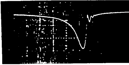
(10 \mu\text{sec} /horizontal division = 0.296 MHz/division) Fig. 61a. Transmitted microwave power vs frequency at 1.7 W.
