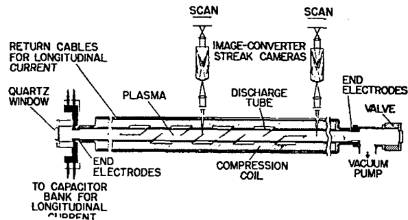
Fig. 3. Scylla IV-3 coil with \ell = 1 grooves and end electrodes
