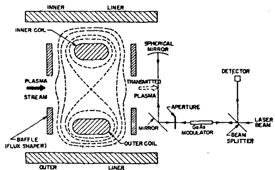
Fig. 45. The interferometer arrangement used for observing gun plasma that was not trapped by the quadrupole field.
