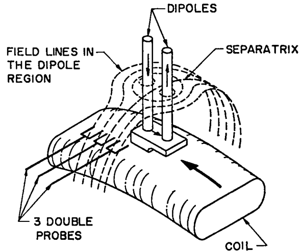
Fig. 50. Schematic diagram showing the position of the double probes used for the electric field measurements in the dipole region. The unguarded protruding dipole crossover piece is also shown.
