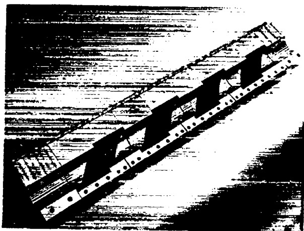
Fig. 1. Portion of Scylla IV-3 compression coil showing \ell = 1 helical groove and Inconel inserts.
