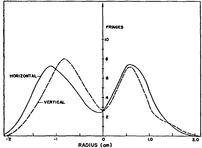
Fig. 9. Density profiles from interferograms of Fig. 7.
