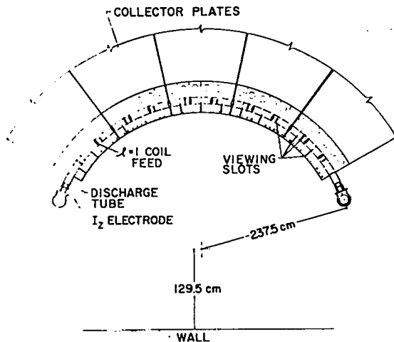
Fig. 23. Top view of compression coil and discharge tube of 5-meter Scyllac toroidal sector.
