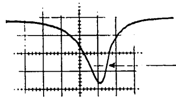
(10 \mu\text{sec} /horizontal division = 0.296 MHz/division) Fig. 62b. Transmitted microwave power vs frequency at 0.15 W.
