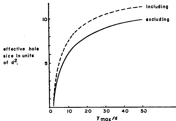
Fig. 53. Effective hole size as a function of the maximum y/d to which the dl integration was taken. For the dotted curve the integration is taken all the way into the nulls so that the non-adiabatic region is included. For the solid curve the non-adiabatic region has been excluded.
