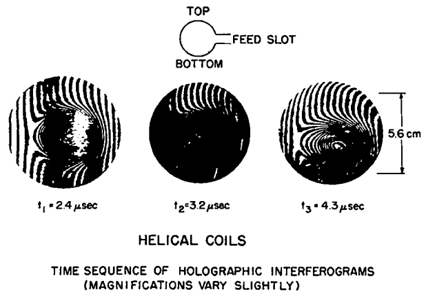
Fig. 18. 3-laser holographic interferograms of Scylla IV-3 with helical l = 1 coils.
